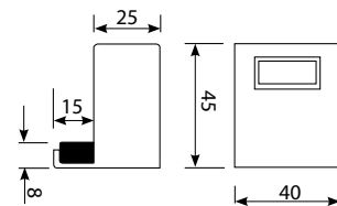
T263 - Deluxe Box Keep/Buffer Suitable for 20mm board To be used with surface fix indicator bolts, open in doors Wood screws supplied Finish: SSS, PSS
