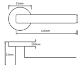
S22-R-SC ARIZONA LEVER ON ROSE SC OTHER FINISHES: PC MATCHING WC TURN: S2-WC-R-SC MATCHING KEY ESC: S2-ESC-KR-SC MATCHING EURO ESC: S2-ESC-ER-SC
