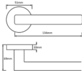
OE-173-AB ROCHESTER LEVER ON ROSE AB OTHER FINISHES: CP MATCHING WC TURN: OE-WC-AB MATCHING KEY ESC: OE-ESC-K-AB MATCHING EURO ESC: OE-ESC-E-AB
