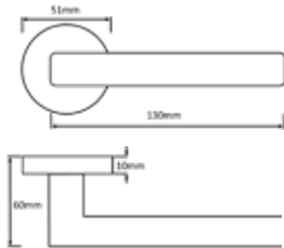
S21-R-SC NEVADA LEVER ON ROSE SC OTHER FINISHES: PC MATCHING WC TURN: S2-WC-R-SC MATCHING KEY ESC: S2-ESC-KR-SC MATCHING EURO ESC: S2-ESC-ER-SC
