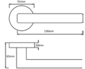
M-73-SN/CP ORAN LEVER ON ROSE SN/CP OTHER FINISHES: N/A MATCHING WC TURN: M-WC-SN/CP MATCHING KEY ESC: M-ESC-K-SN/CP MATCHING EURO ESC: M-ESC-E-SN/CP
