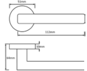
OE-177-AB COLCHESTER LEVER ON ROSE AB OTHER FINISHES: DS, MBN MATCHING WC TURN: OE-WC-AB MATCHING KEY ESC: OE-ESC-K-AB MATCHING EURO ESC: OE-ESC-E-AB
