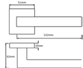
S23-S-SC CALIFORNIA LEVER ON ROSE SC OTHER FINISHES: N/A MATCHING WC TURN: S2-WC-S-SC MATCHING KEY ESC: S2-ESC-KS-SC MATCHING EURO ESC: S2-ESC-ES-SC
