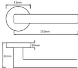
M-53-SN/NP MESSINA LEVER ON ROSE SN/NP OTHER FINISHES: N/A MATCHING WC TURN: M-WC-SN/NP MATCHING KEY ESC: M-ESC-K-SN/NP MATCHING EURO ESC: M-ESC-E-SN/NP
