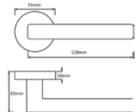
M-62-SN/NP NAPLES LEVER ON ROSE SN/NP OTHER FINISHES: N/A MATCHING WC TURN: M-WC-SN/NP MATCHING KEY ESC: M-ESC-K-SN/NP MATCHING EURO ESC: M-ESC-E-SN/NP
