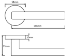
M-78-SN/CP MONACO LEVER ON ROSE SN/CP OTHER FINISHES: N/A MATCHING WC TURN: M-WC-SN/CP MATCHING KEY ESC: M-ESC-K-SN/CP MATCHING EURO ESC: M-ESC-E-SN/CP
