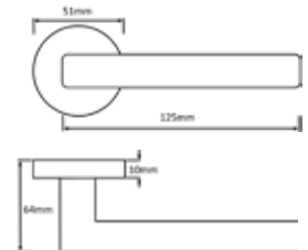
M-125-SN/CP TUNIS LEVER ON ROSE SN/CP OTHER FINISHES: N/A MATCHING WC TURN: M-WC-SN/CP MATCHING KEY ESC: M-ESC-K-SN/CP MATCHING EURO ESC: M-ESC-E-SN/CP
