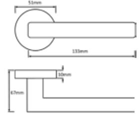
M-46-SN/NP IBIZA LEVER ON ROSE SN/NP OTHER FINISHES: N/A MATCHING WC TURN: M-WC-SN/NP MATCHING KEY ESC: M-ESC-K-SN/NP MATCHING EURO ESC: M-ESC-E-SN/NP
