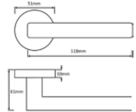
S35-R-PC TEXAS LEVER ON ROSE PC OTHER FINISHES: SC MATCHING WC TURN: S2-WC-R-PC MATCHING KEY ESC: S2-ESC-KR-PC MATCHING EURO ESC: S2-ESC-ER-PC
