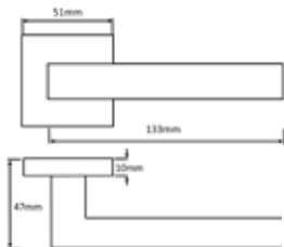
S24-S-PC KANSAS LEVER ON ROSE PC OTHER FINISHES: SC MATCHING WC TURN: S2-WC-S-PC MATCHING KEY ESC: S2-ESC-KS-PC MATCHING EURO ESC: S2-ESC-ES-PC
