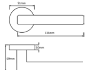
OE-173-CP ROCHESTER LEVER ON ROSE CP OTHER FINISHES: AB MATCHING WC TURN: OE-WC-CP MATCHING KEY ESC: OE-ESC-K-CP MATCHING EURO ESC: OE-ESC-E-CP
