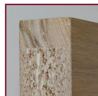
Side view of lipping and core
