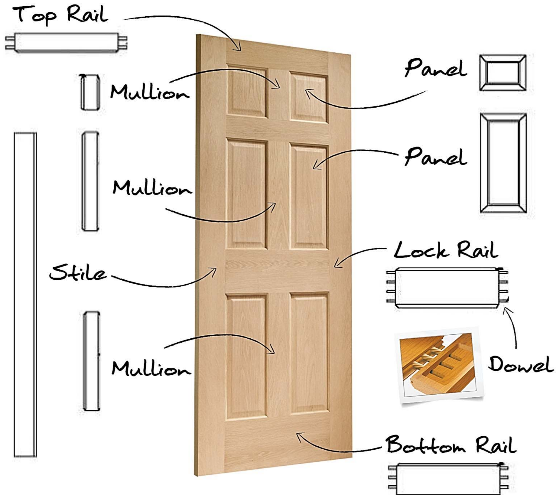
Door Components
