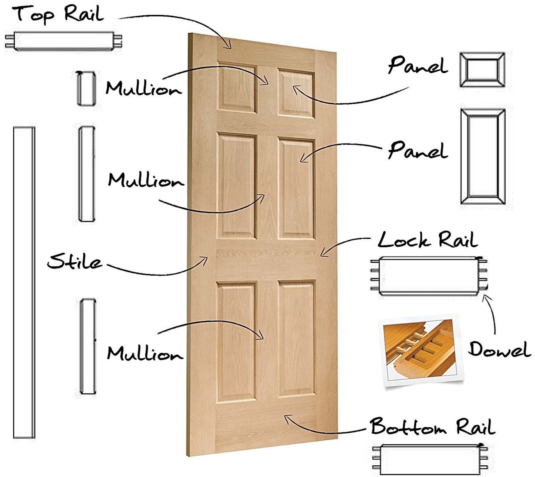
Door Components
